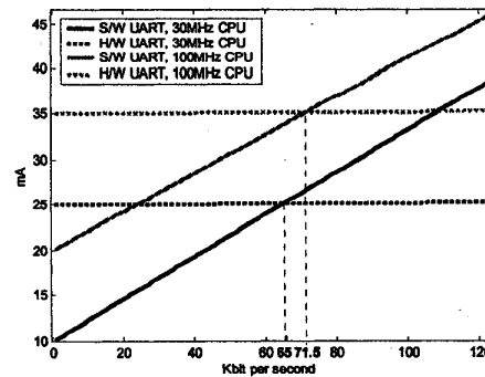
Figure 3. Power consumption curves
